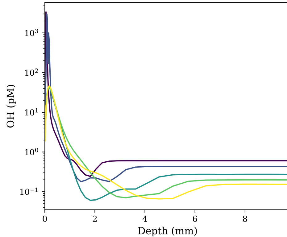
(e) OH
