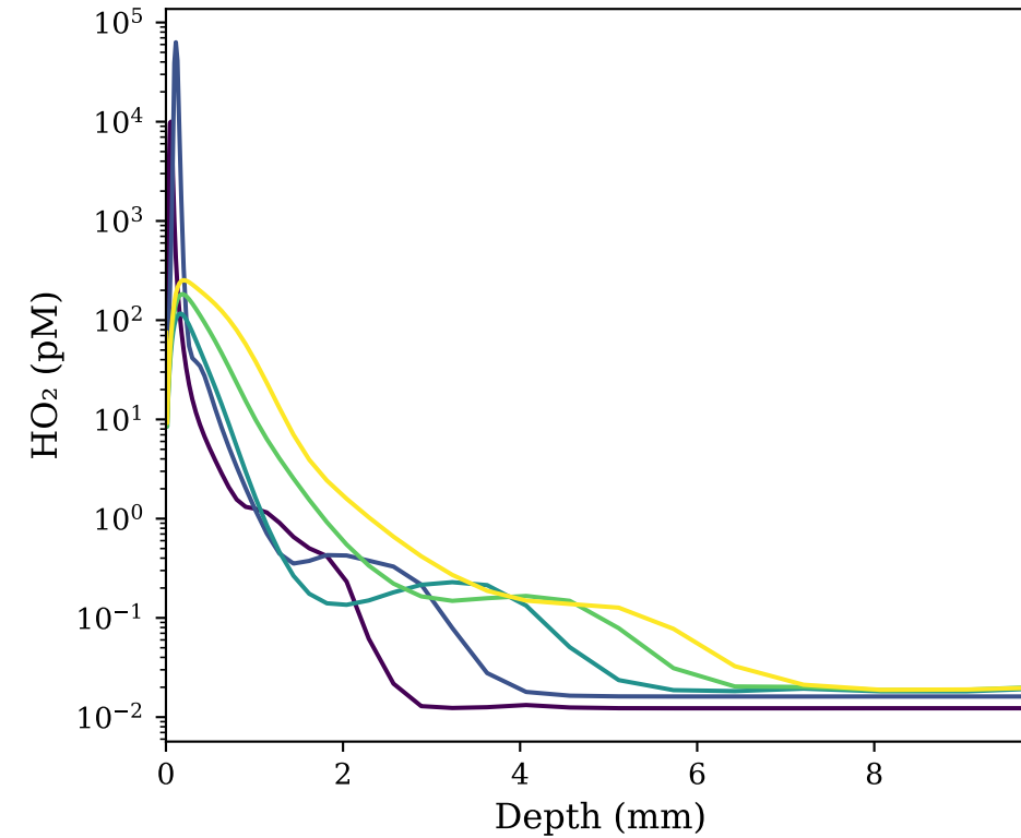
(f) \text{HO}_2
